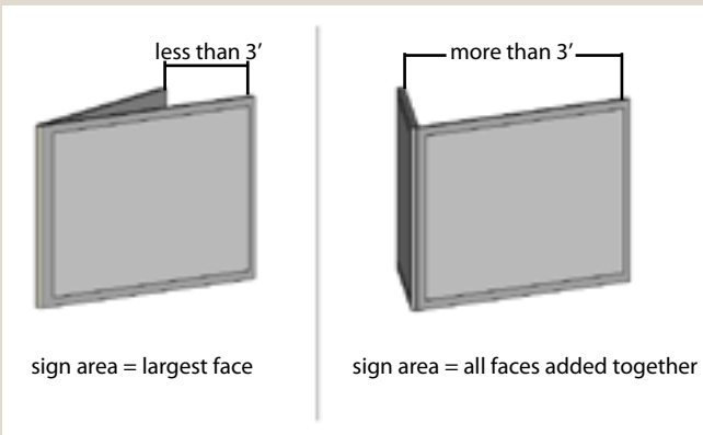
Figure 1-8: Double-faced Sign
